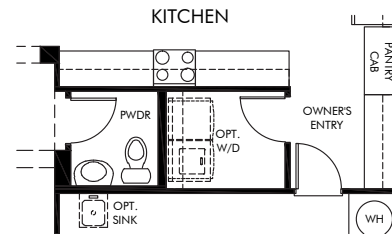
OPT. POWDER BATH ILO STORAGE
