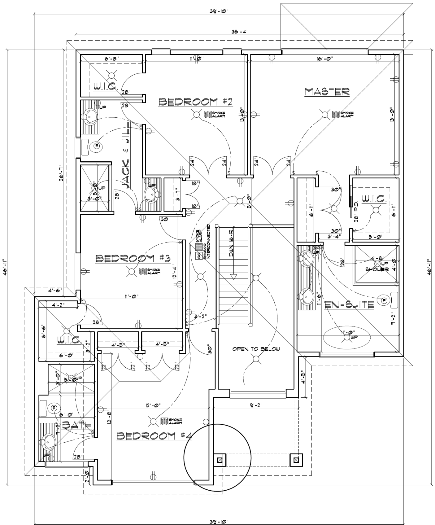
(ROOF LINES FOR ELEVATION AA-1) "DUBLIN" CONTEMPORARY SECOND FLOOR PLAN APPROX.-1494 (GROSS) SQ. FT. APPROX.-1391 (NET) SQ. FT.
