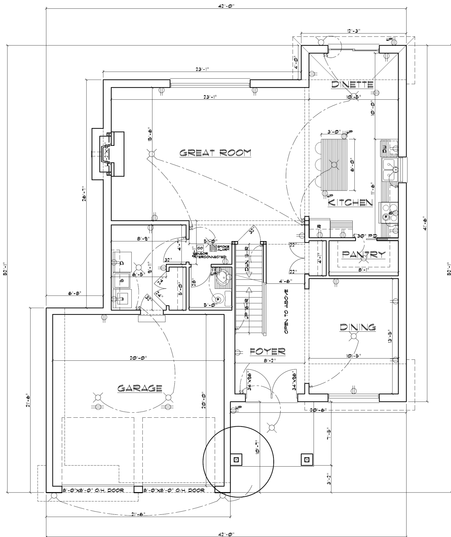
(ROOF LINES FOR ELEVATION AA-1) "DUBLIN" CONTEMPORARY FIRST FLOOR PLAN (STANDARD) APPROX.-1249 SQ. FT.
