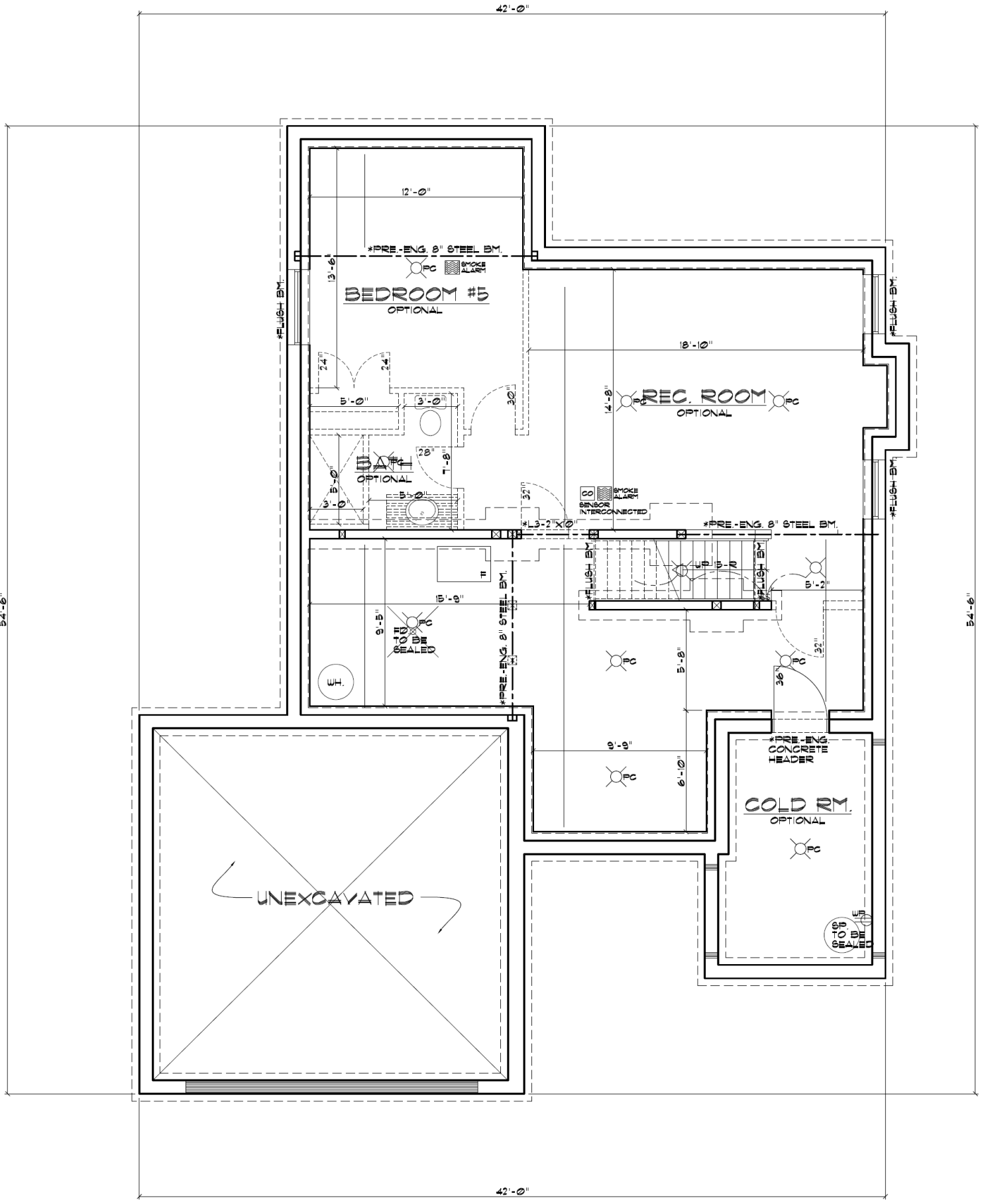
(FOUNDATION LAY OUT FOR AA-1,2) "GALWAY" TRADITIONAL FOUNDATION PLAN APPROX. - 657 SQ. FT. OF (OPTIONAL) FINISHED BASEMENT
