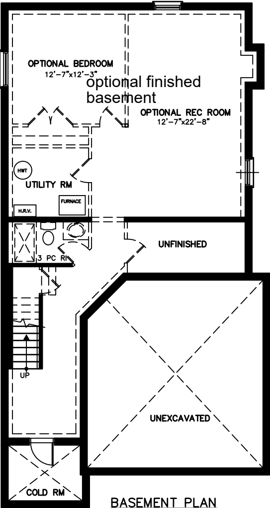
BASEMENT PLAN OPTIONAL FINISHED AREA 961 sq.ft.
