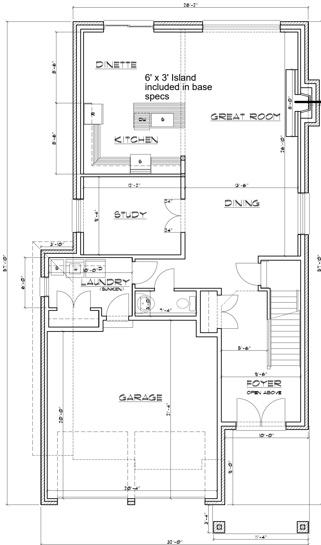
"STEEL ORANGE" CONTEMPORARY FIRST FLOOR PLAN APPROX. - 1204 SQ. FT.
