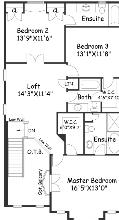
Second Floor Plan (3 Bedrooms + Loft)
