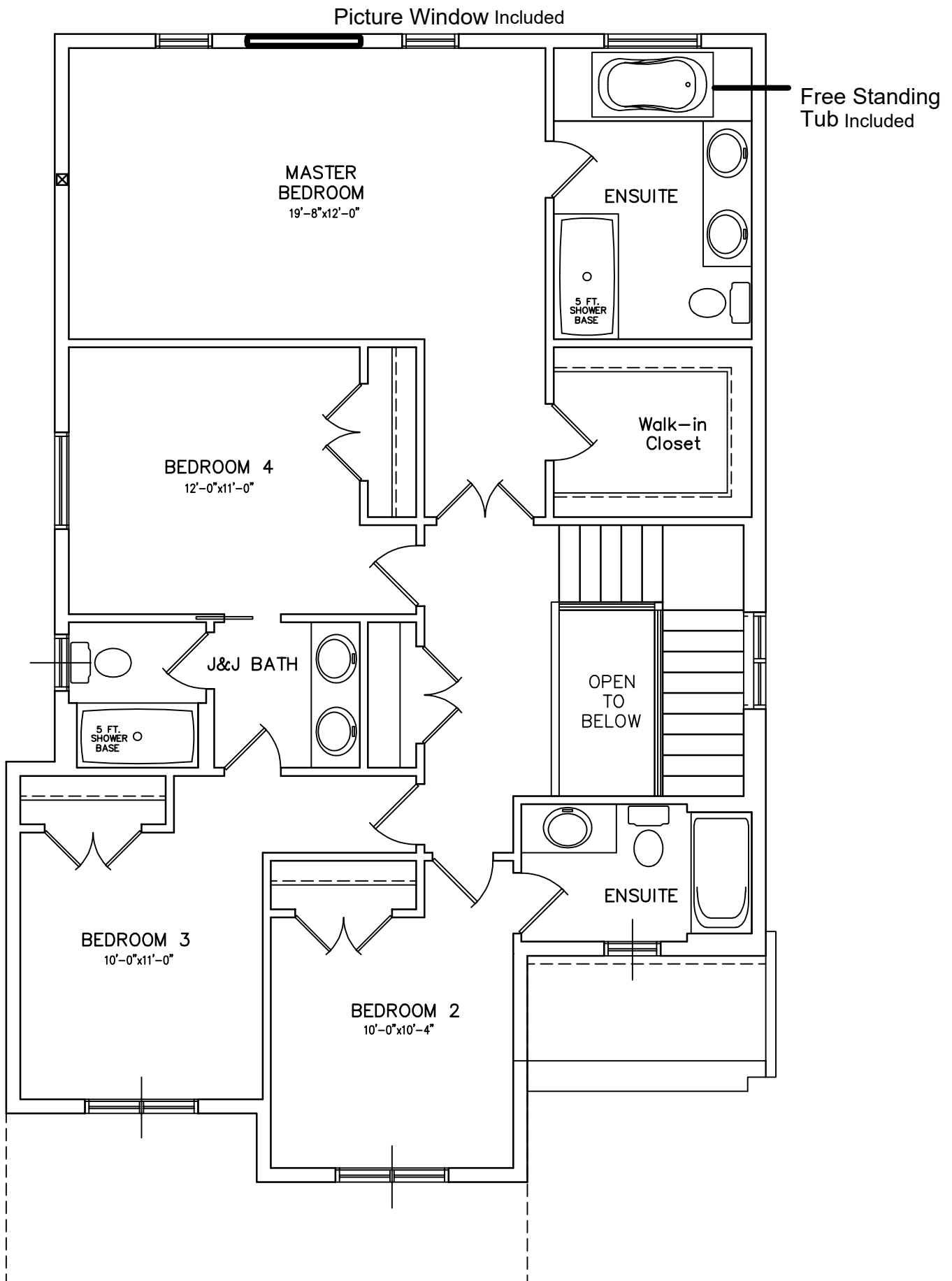
SECOND FLOOR PLAN – 1272 sq.ft. PLUS 30 SQ.FT. SPACE OPEN TO BELOW
