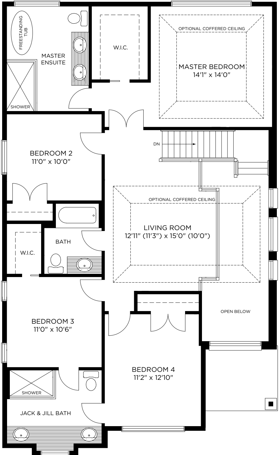
SECOND FLOOR PLAN - OPTION 2
