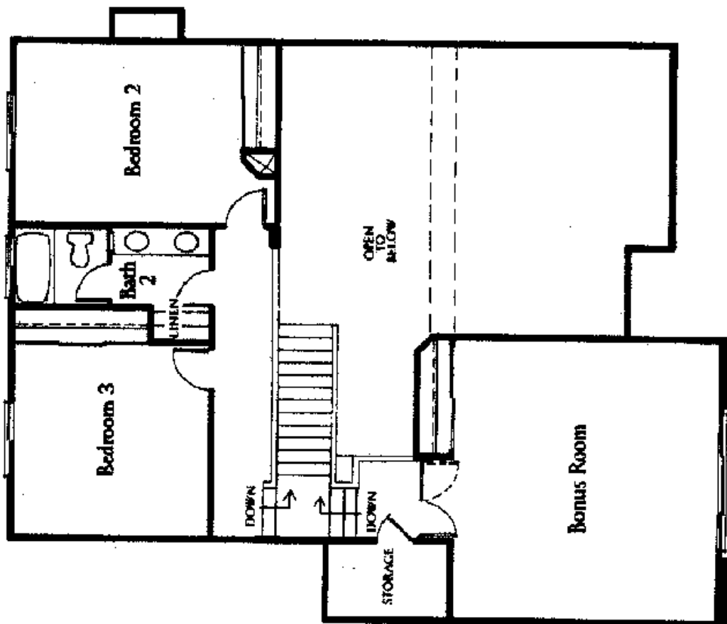
SECOND FLOOR
