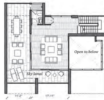
Upper level 5
