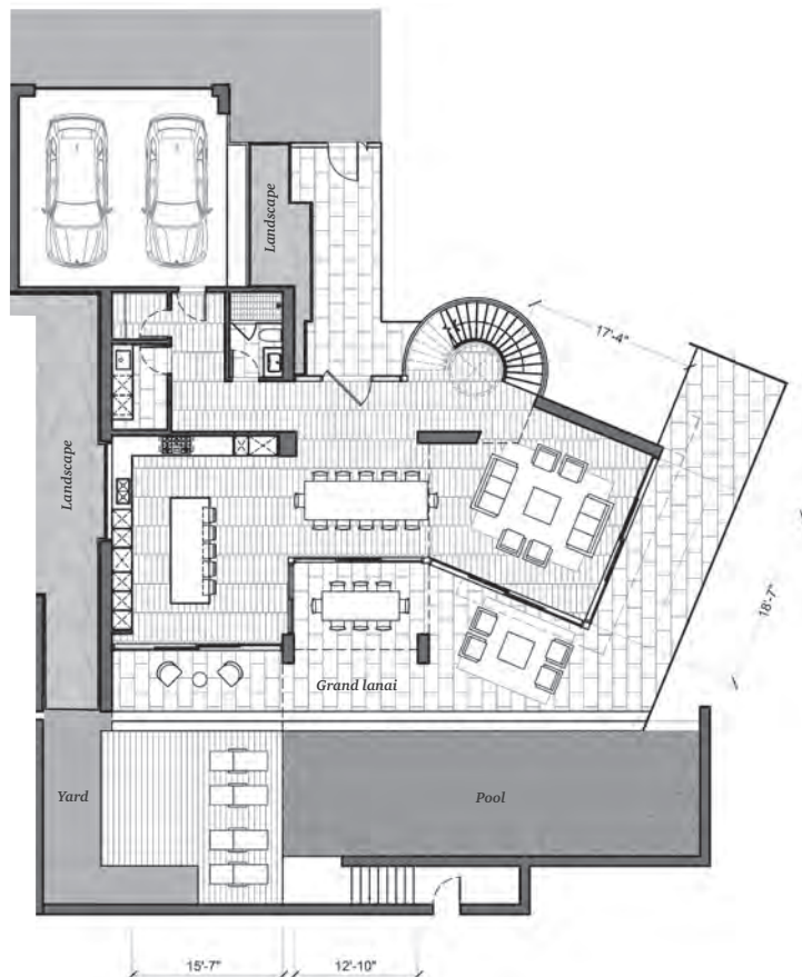
Ground level 1
