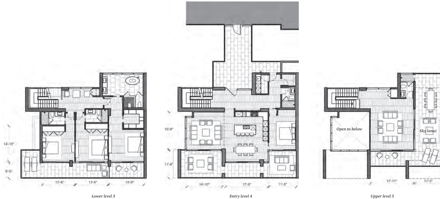
Lower level 3
