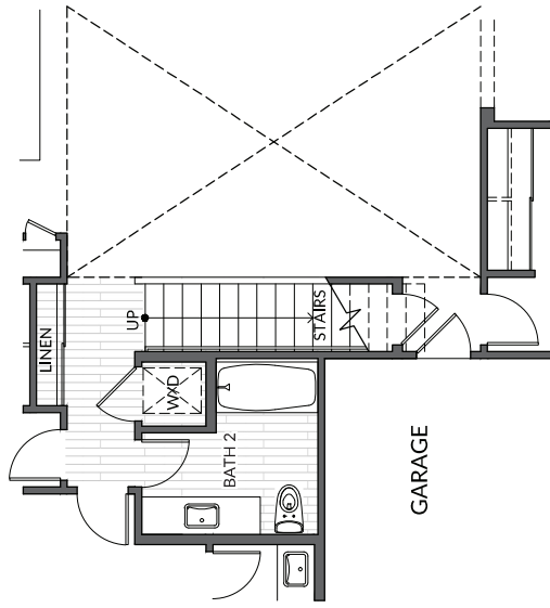
STAIRS TO LOFT Plan A2 Option
