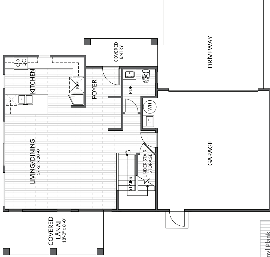
LOWER FLOOR
