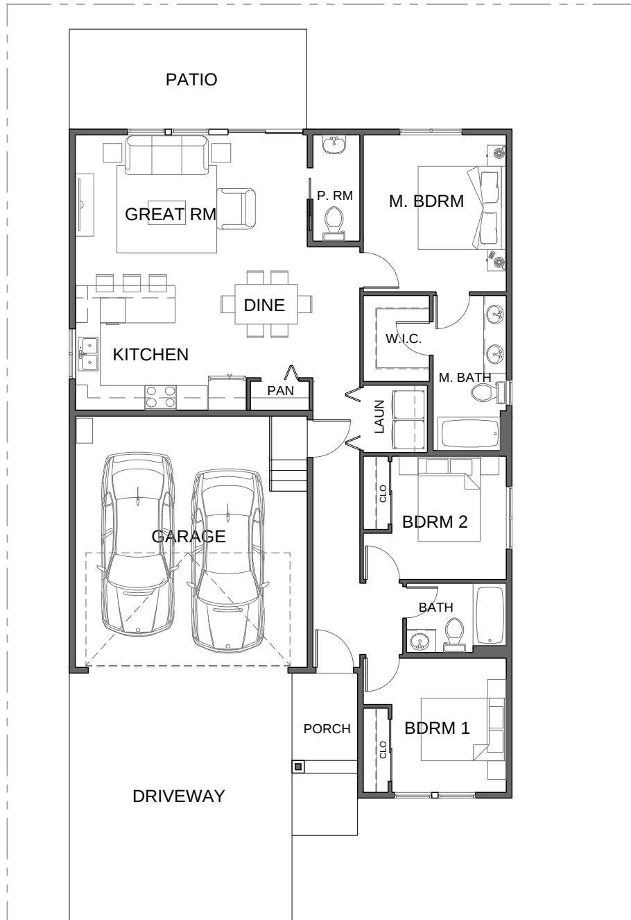
FLOOR PLAN L - 1,266 SF
