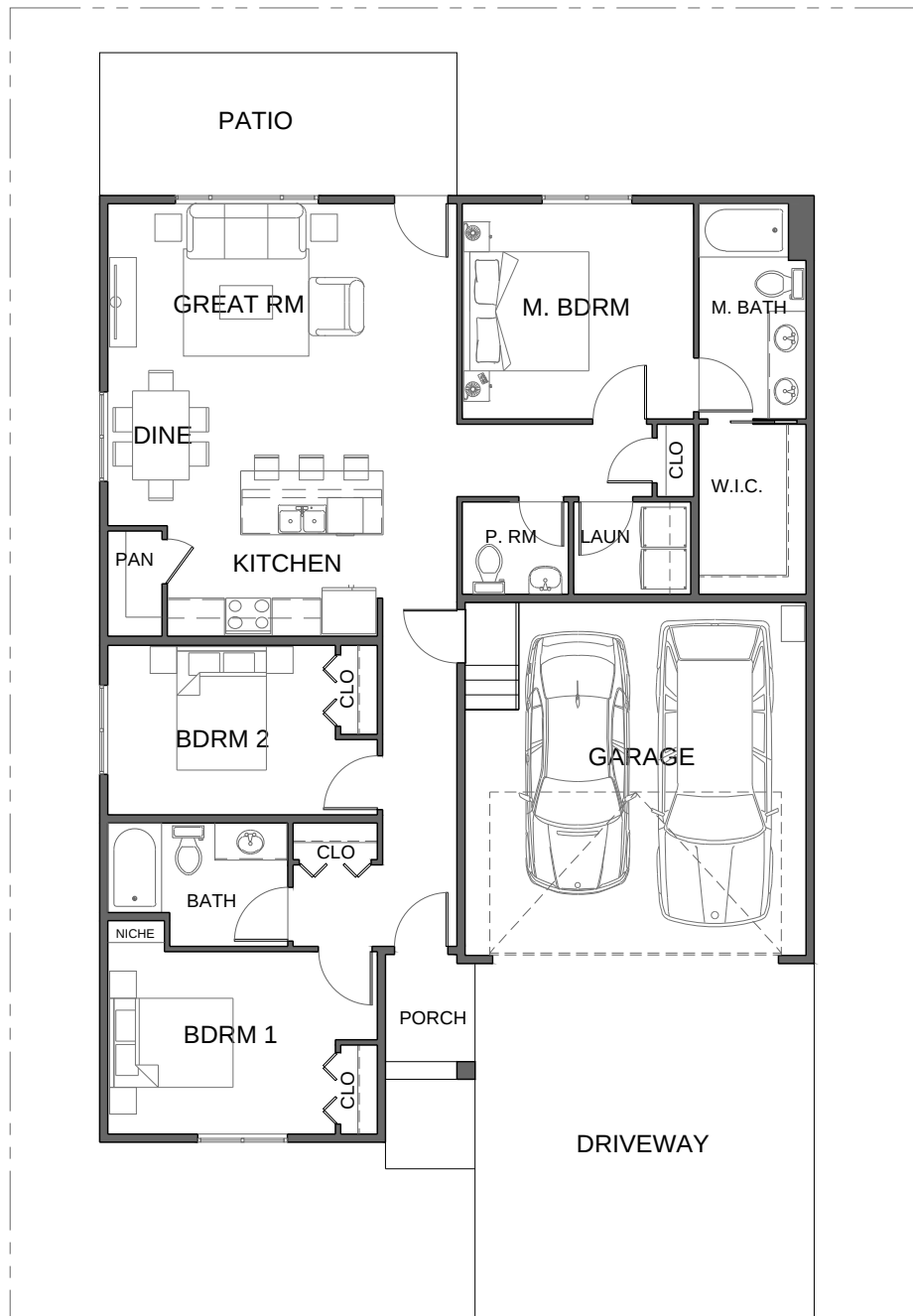
FLOOR PLAN R - 1,474 SF
