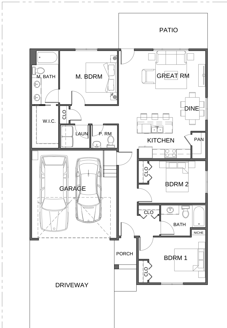
FLOOR PLAN L - 1,474 SF
