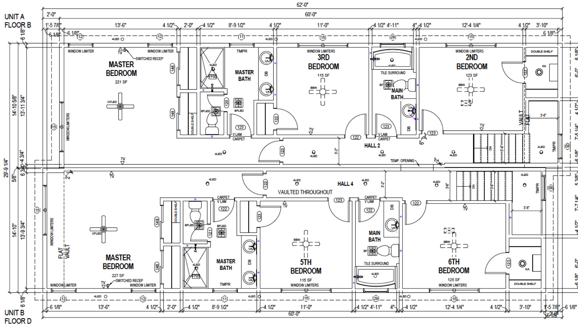
1 2ND FLOOR PLAN 01B SCALE (22x34): 3/8" = 1'-0" SCALE (11x17): 3/16" = 1'-0"
