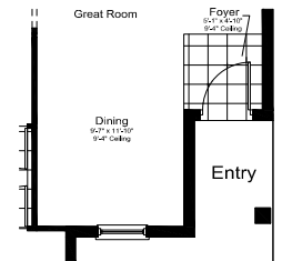
Dining I/O Den w/ No Column or Soffit at Foyer elevation I-1 shown, windows vary per elevation
