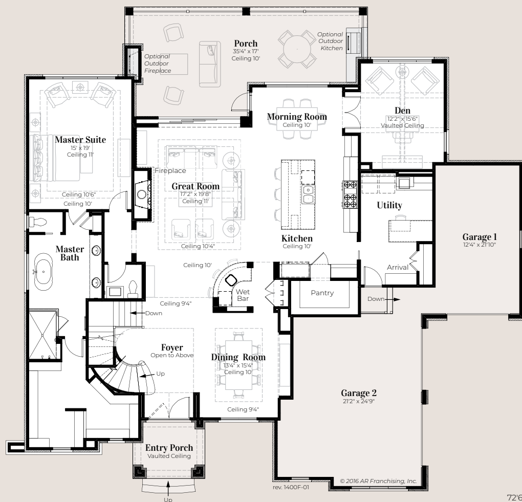
Main Level
