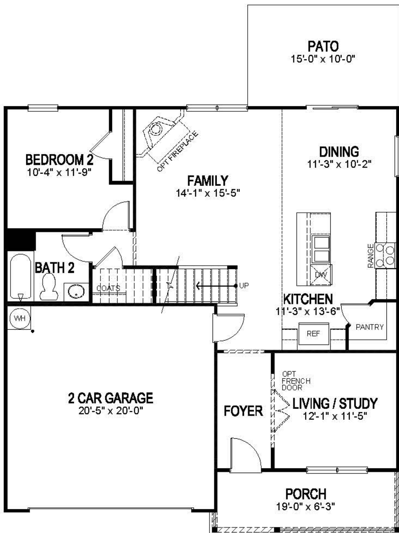
FIRST FLOOR
