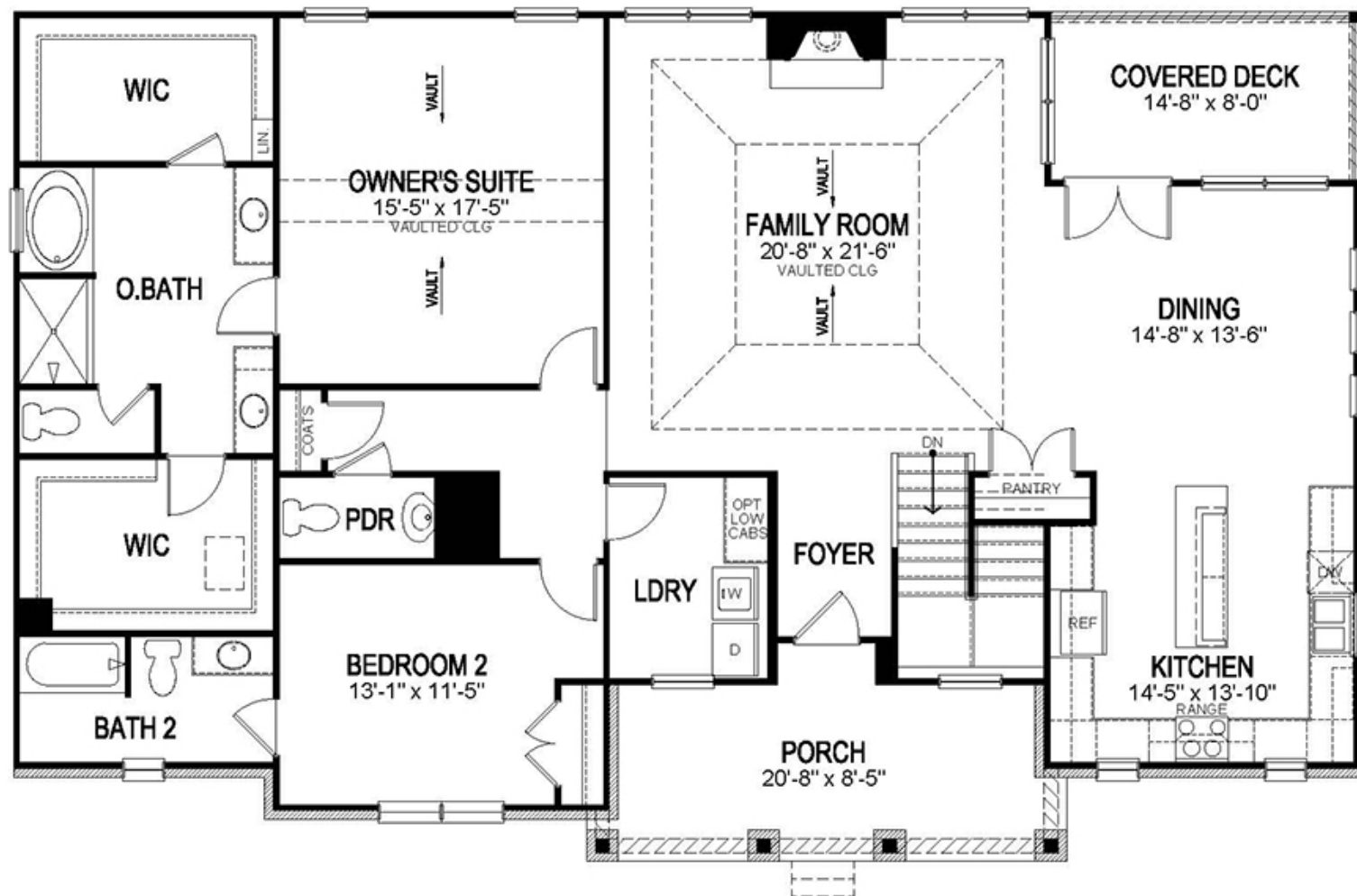
FIRST FLOOR
