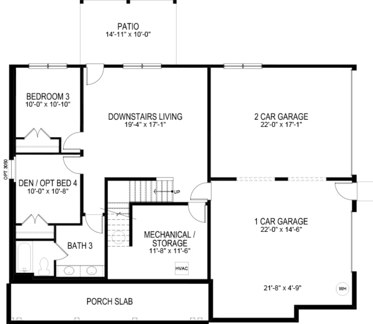
WALKOUT BASEMENT
