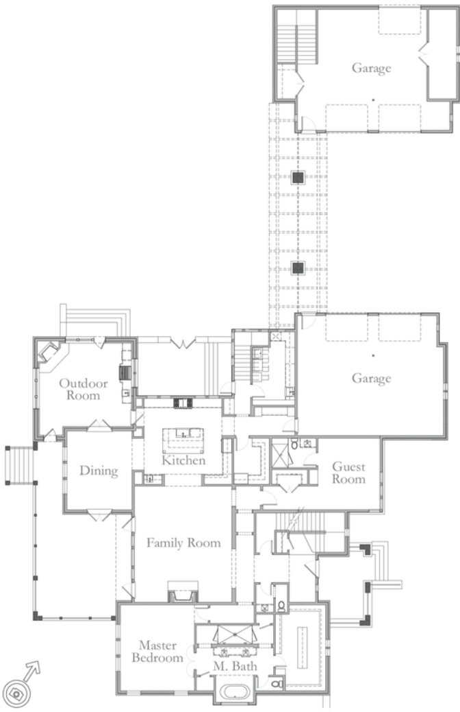
MAIN FLOOR 3,602 sf
