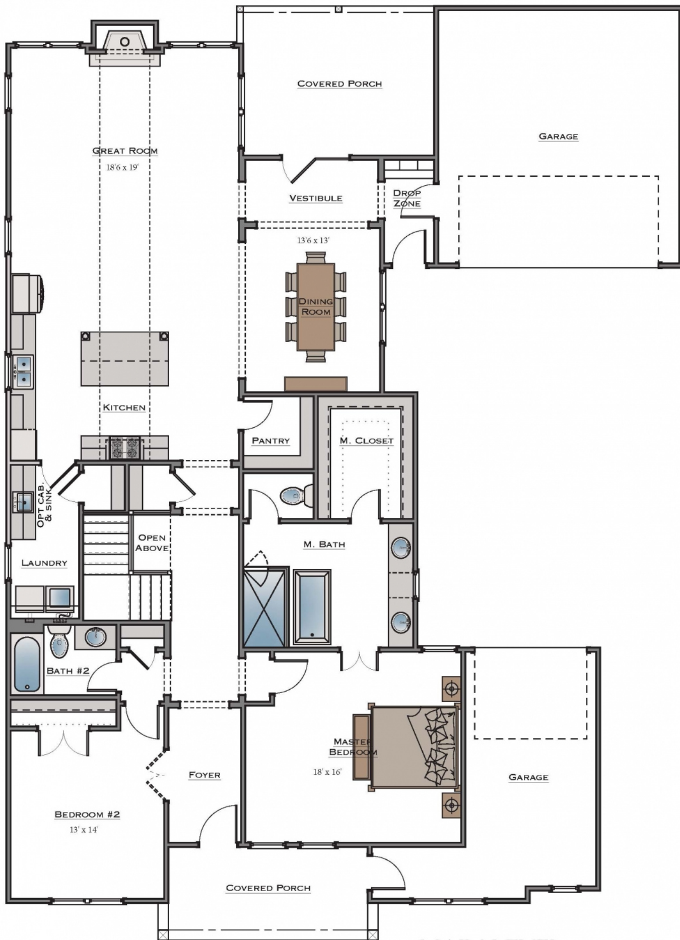
MAIN LEVEL
