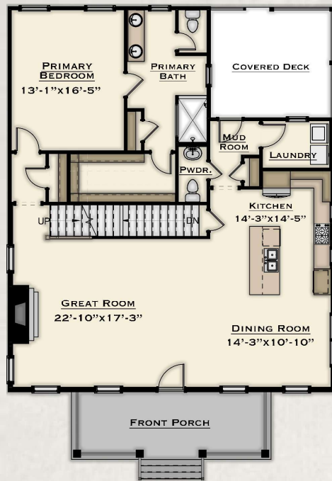
Main Level
