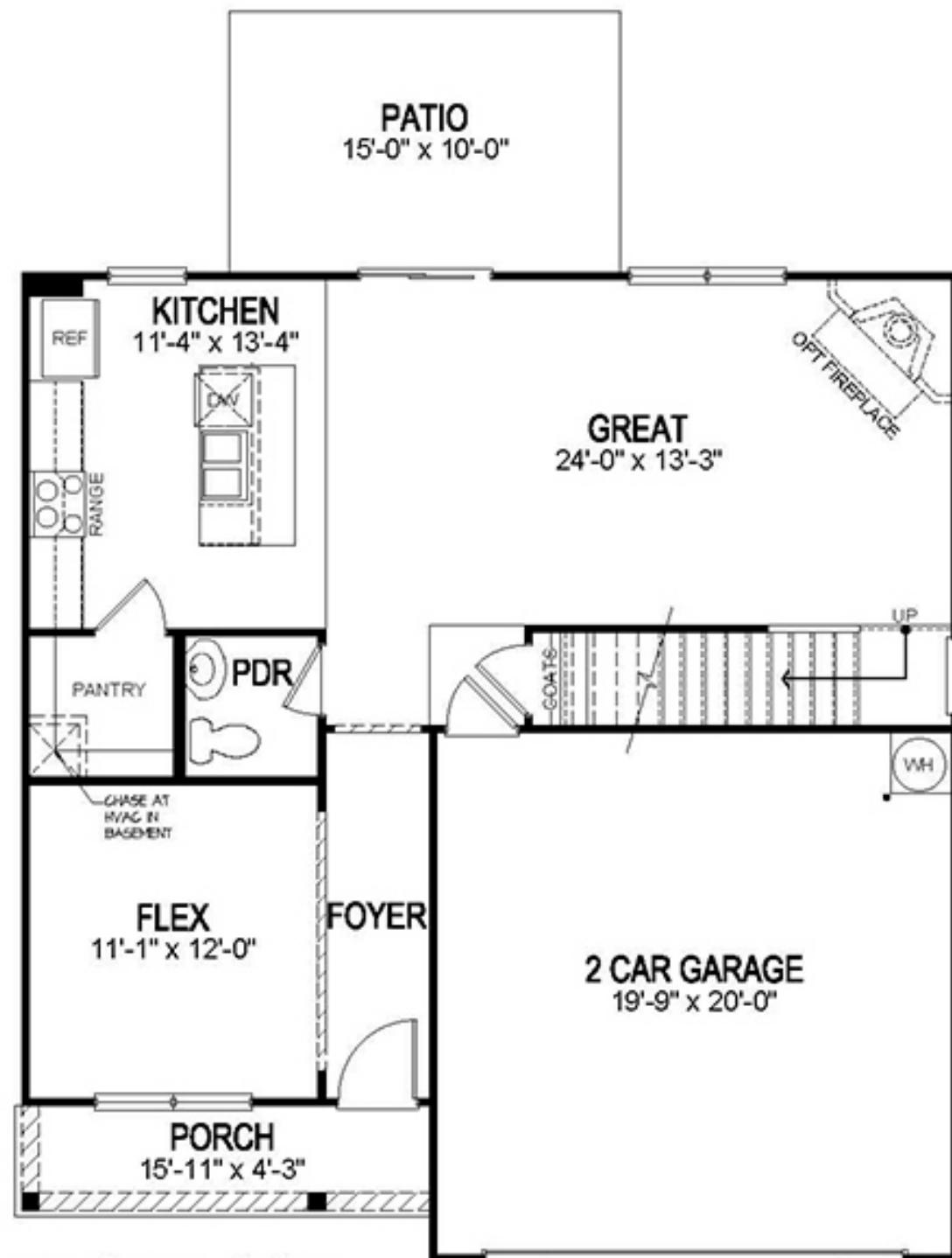
FIRST FLOOR
